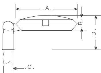
Pole Mount
